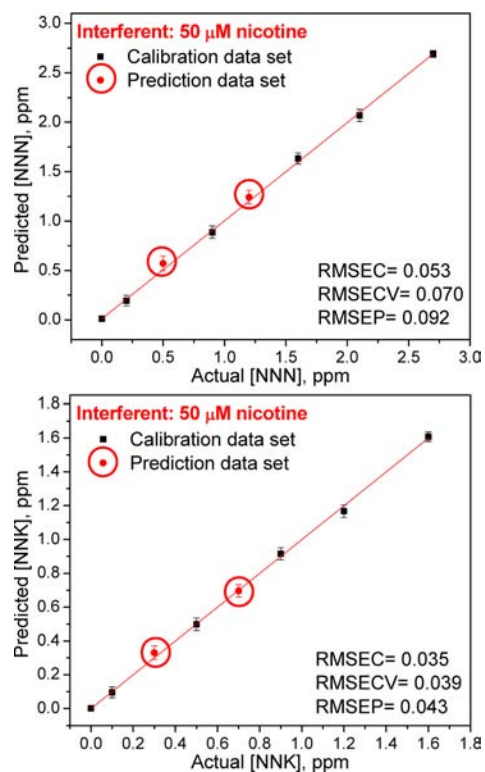
Figure 6. Results of the SVM regression for quantitative analysis of (top) NNN and (bottom) NNK mixtures in the presence of interfering nicotine ( 50 \mu\text{M} ). The plots of actual vs predicted concentration show high accuracy of prediction for multiple guest concentrations. The values of the root-mean-square errors (RMSEs) of calibration (C), cross-validation (CV), and prediction (P) (shown as insets) attest to the high quality of the model and prediction.
