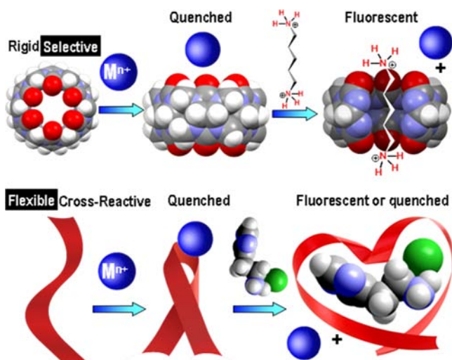
Figure 2. Probes 1 and 2 are fluorescent, and their fluorescence is partly quenched by the bound metal ion. Depending on the guest structure, the interaction between the probe and the guest results in either recovery or further quenching of the fluorescence. Probes 1 and 2 utilize complementary features of selective probe 1, which has a narrow cavity displaying a preference for aliphatic guests, and flexible probe 2, which adapts its size to a wider variety of guests.
